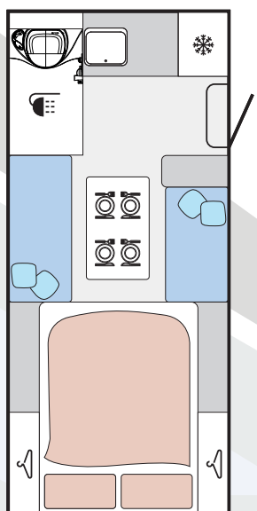
HYBRID 480 LAYOUT 2
