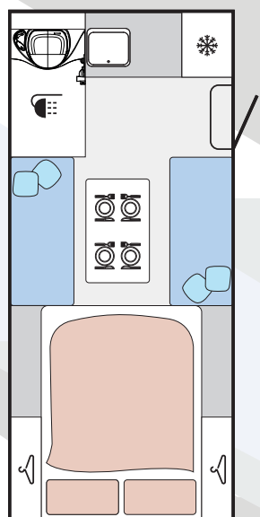
HYBRID 480 LAYOUT 1
