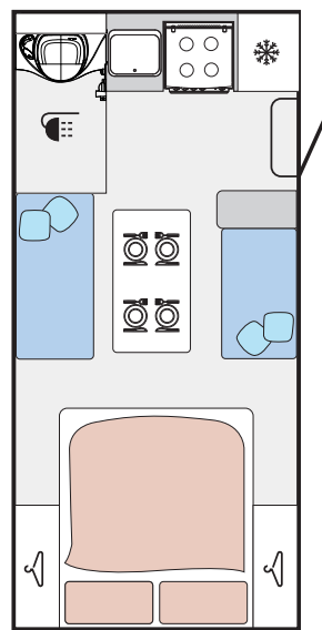
SIERRA 480 LAYOUT 3
