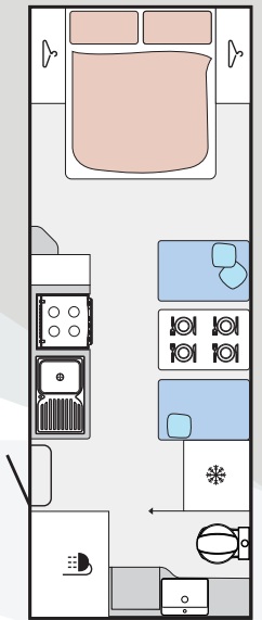
595 BLACKHAWK LAYOUT 1
