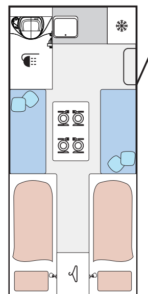
HYBRID 480 LAYOUT 4
